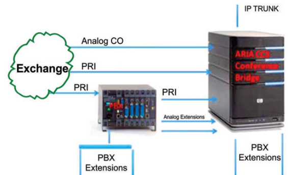
ARIA ACCS - CONFERENCE BRIDGE - NETWORK DIAGRAM
