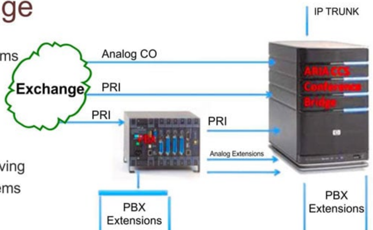
ARIA ACCS - CONFERENCE BRIDGE - NETWORK DIAGRAM
